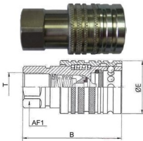
Poppet Type
