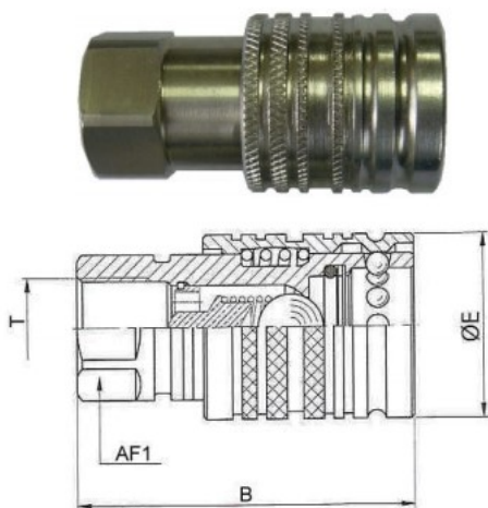
Ball Type
